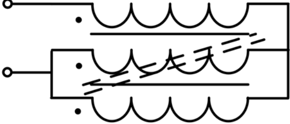
Differential Mode
