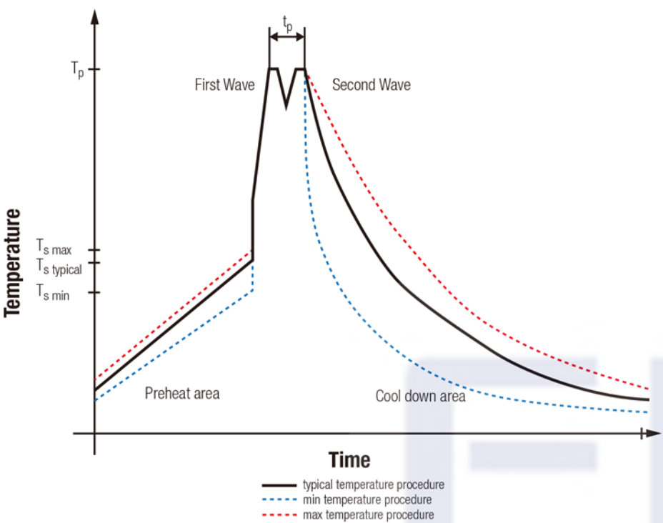
Classification Wave Soldering Profile:
