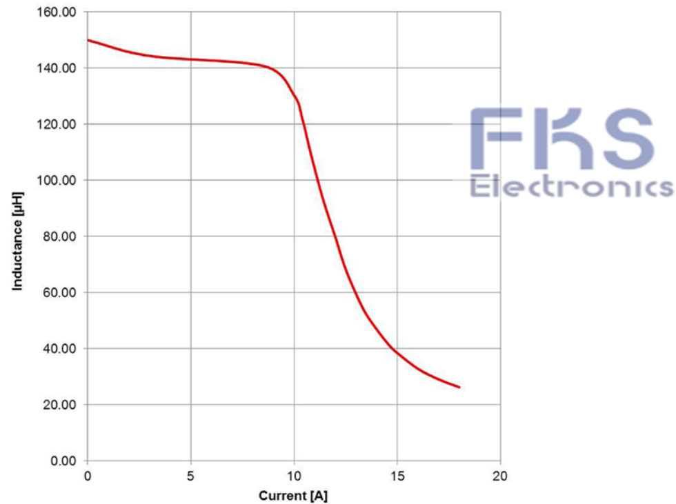
F1 Typical Inductance vs. Current Characteristics:
