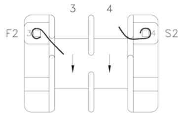
COIL 2
